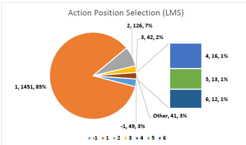
Figure 6.7. Action Position Selection (LMS).
