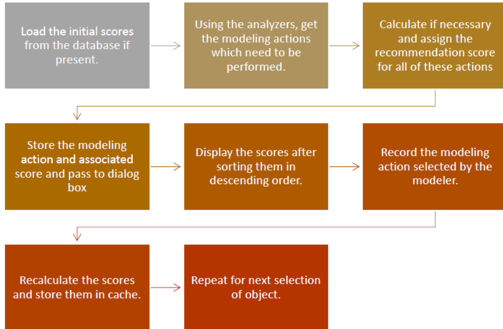
Figure B.5. Calculation of Scoring Mechanism.
