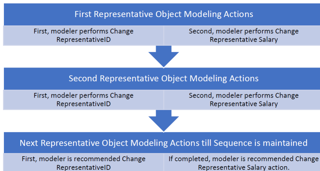
Figure 5.4. Sequence Recommendation Demonstration.
