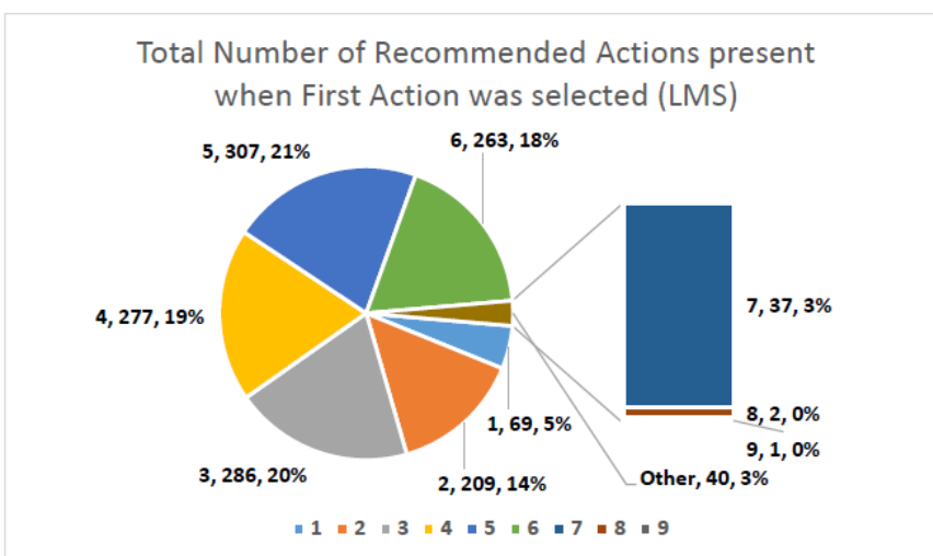
Figure 6.8. First Action Selection (LMS).
