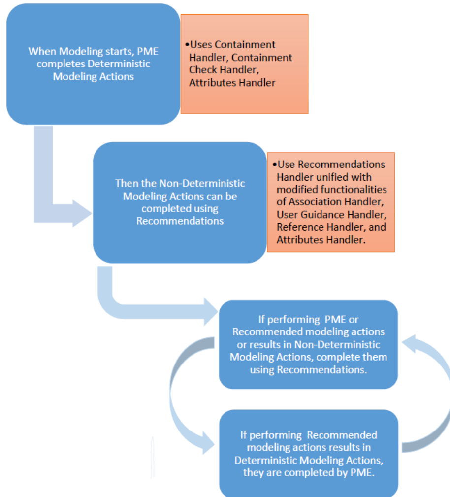
Figure 4.1. Recommender System integrated in Proactive Modeling Working
