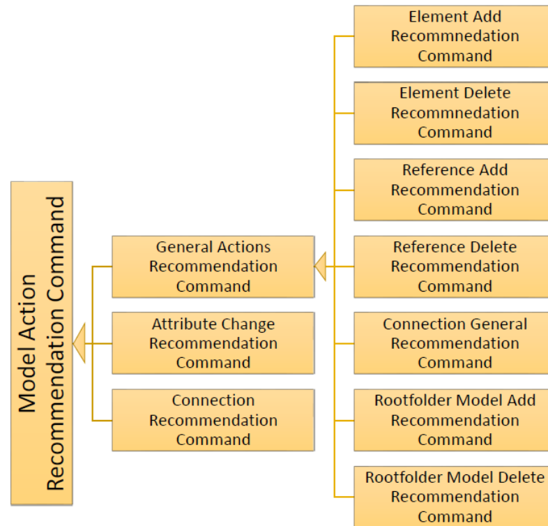
Figure B.2. Model Action Recommendation Command Hierarchy.
