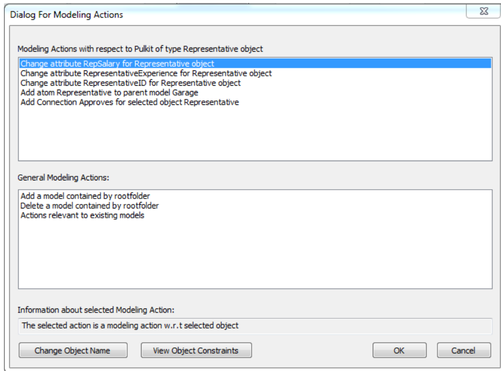
Figure 5.1. Recommendation Dialog Box to display Modeling Actions.
