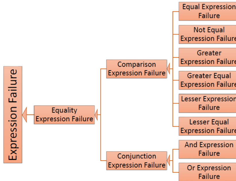
Figure B.1. Expression Failure Hierarchy.
