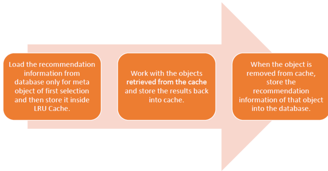
Figure B.4. Optimization of Information using LRU cache.
