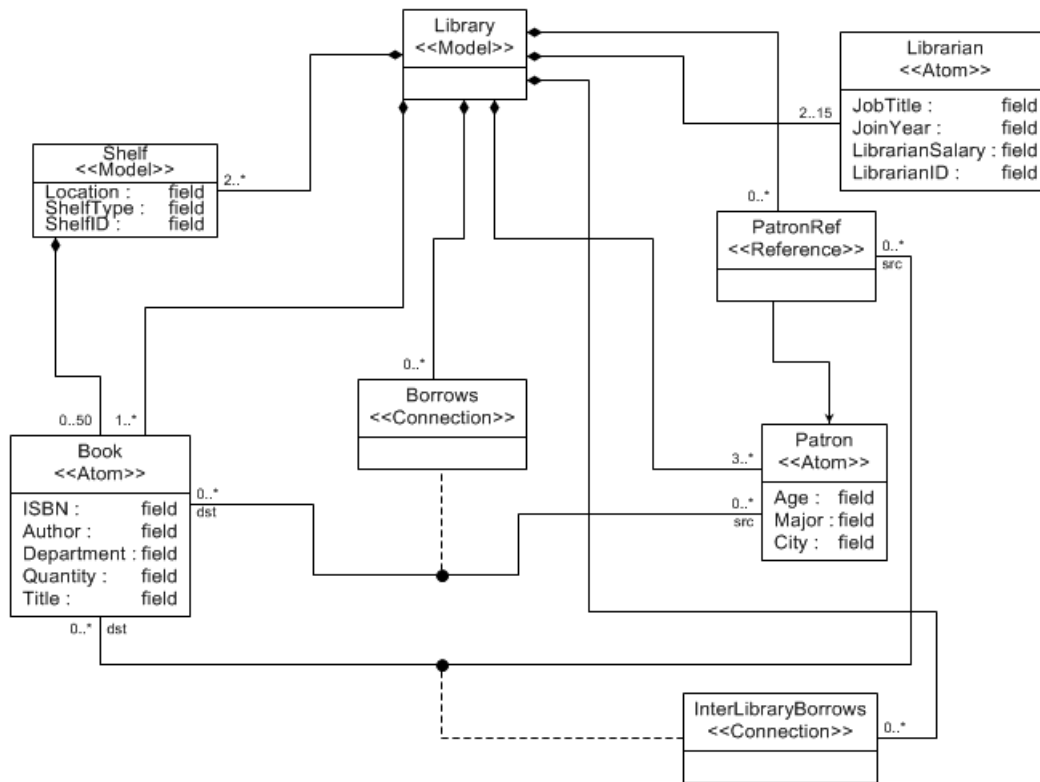
Figure 3.16. A Sample Metamodel for LMS.
