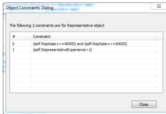
Figure 5.2. View Object Constraints.
