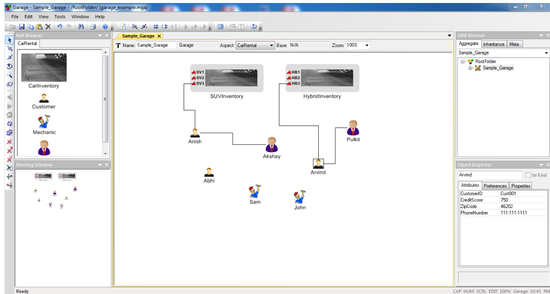
Figure 3.15. A example model created from the CRS metamodel.
